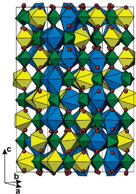
Figure 4. The crystal structure of \alpha - \text{K}_3\text{AlF}_6 . The \text{AlF}_6 octahedra are green; the \text{K}_\text{B}\text{F}_7 and \text{K}_\text{A}\text{F}_8 polyhedra are yellow and blue, respectively. The \text{K}_\text{A} cations are shown as brown spheres.
