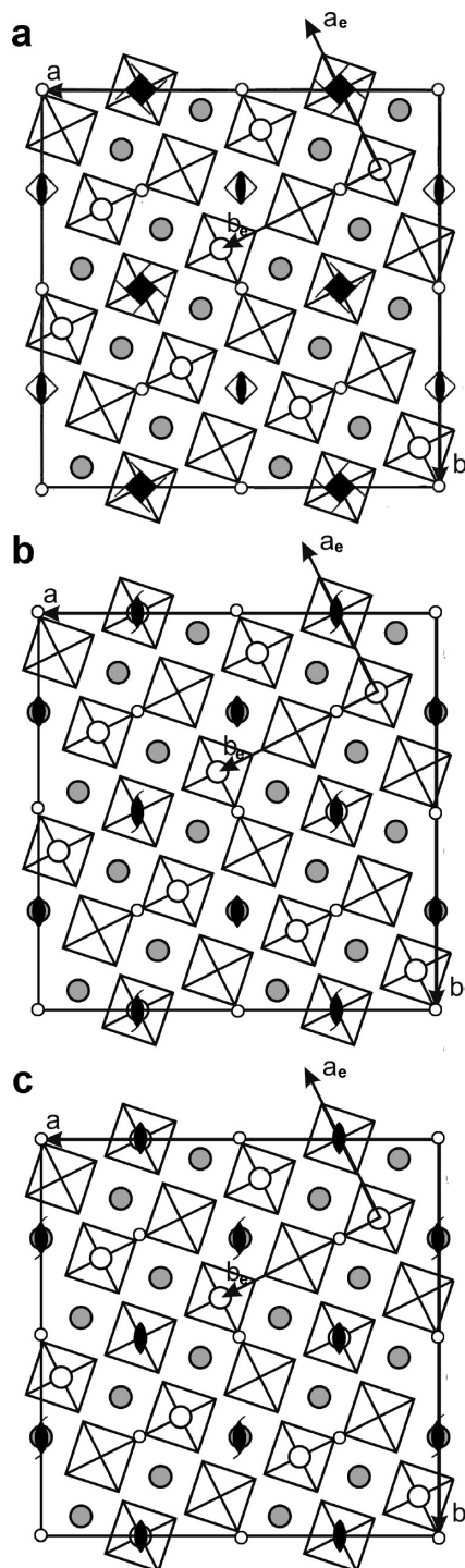
Figure 2. The projection of the parent elpasolite structure within the a=b \approx a_c\sqrt{5} , c=4a_c supercell with overlaid positions of symmetry axes and inversion centers of the I4_1/a (a), I12/b (b), and I12/a (c) space groups. The B'X_6 octahedra are shown; the A and B cations are shown as empty and gray circles, respectively. The notations for symmetry elements correspond to those in the International Tables for Crystallography.
