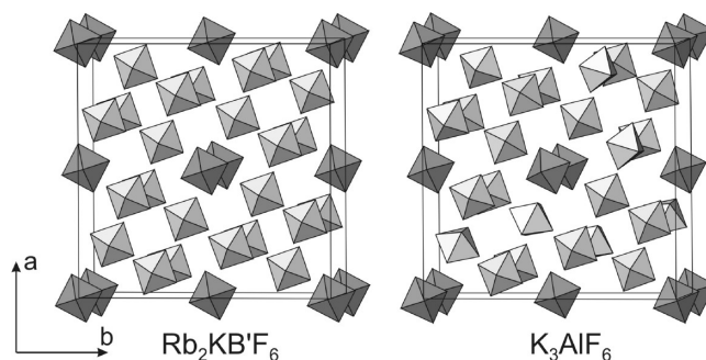
Figure 7. A comparison of the \text{Rb}_2\text{KB}'\text{F}_6 ( \text{B}' = \text{Cr}, \text{Ga} ) and \alpha - \text{K}_3\text{AlF}_6 structures. Both structures are drawn in the F -centered tetragonal a = b \approx a_c\sqrt{5} , c = a_c unit cell. The A and B cations are not shown. The \text{B}'\text{F}_6 and \text{AlF}_6 octahedra rotated over \pi/4 around the c axis are shaded a darker gray.
