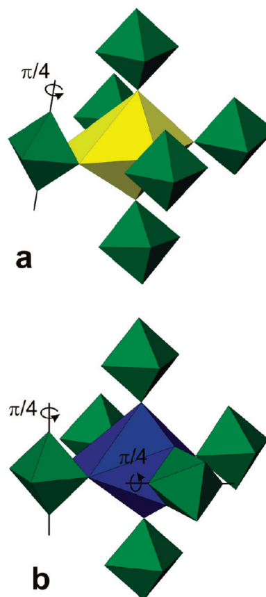
Figure 5. A formation of the \text{K}_\text{B}\text{F}_7 (a) and \text{K}_\text{A}\text{F}_8 (b) polyhedra as a result of rotation of the \text{AlF}_6 octahedra (green) over \sim\pi/4 .
