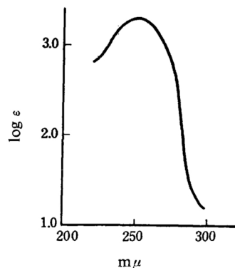
Fig. 7. Ultraviolet absorption spectrum of XXII in water.
