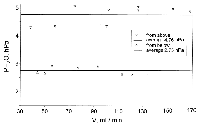
Fig. 6. Water vapour pressure for the system \text{CaCl}_2\text{--CaCl}_2\cdot \text{H}_2\text{O} at 354.30 K.
