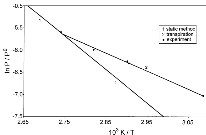
Fig. 11. Water vapour pressure for the system MnCl_2-MnCl_2 \cdot H_2O .
