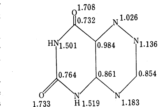
Fig. 3. \pi -Electron Distributions
