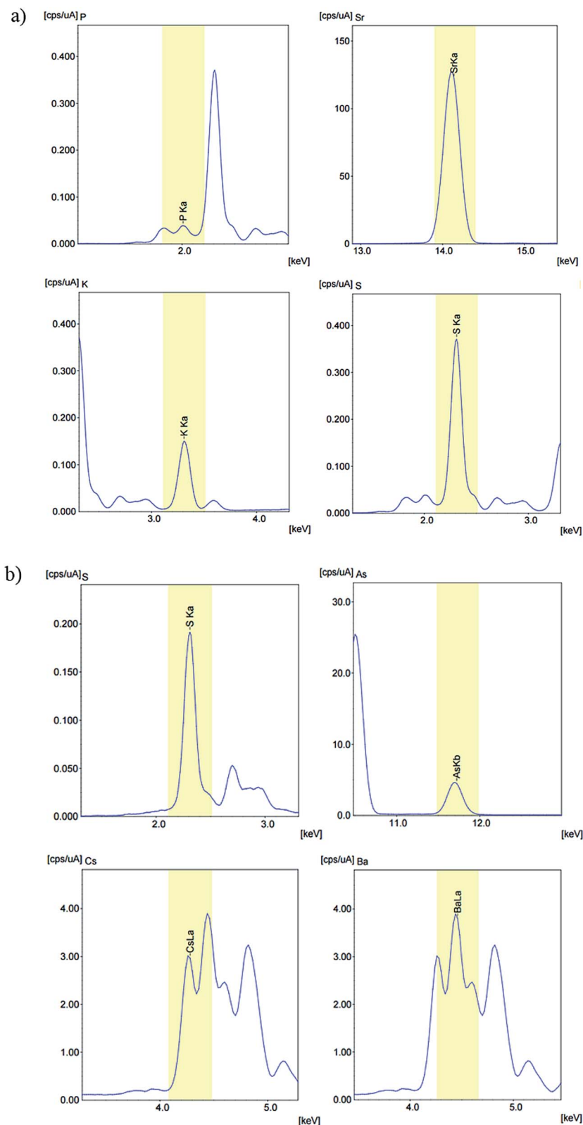
Fig. 1 (a) Energy dispersive X-ray fluorescence spectra of \text{K}_2\text{SrP}_4 , (b) energy dispersive X-ray fluorescence spectra of \text{CsBaAs}_4 .
