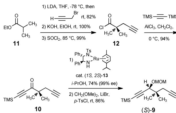
Scheme 2. Preparation of the Key Building Block ( S )- 9
