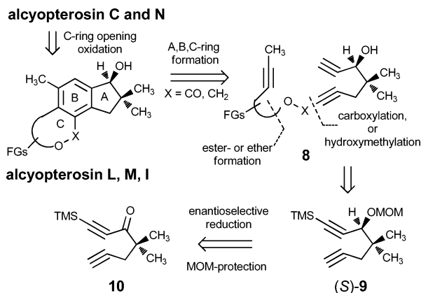
Scheme 1. Retrosynthetic Analysis
