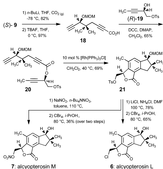
Scheme 4. Synthesis of Alcyopterosin L ( 6 ) and M ( 7 )
