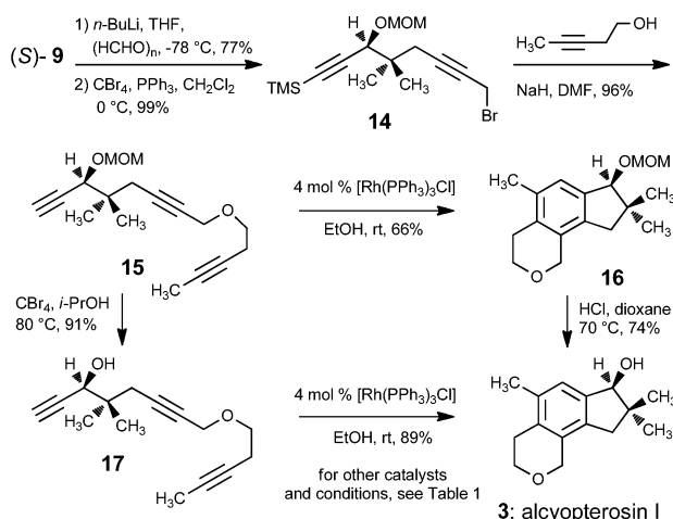
Scheme 3. Synthesis of Alcyopterosin I ( 3 )
