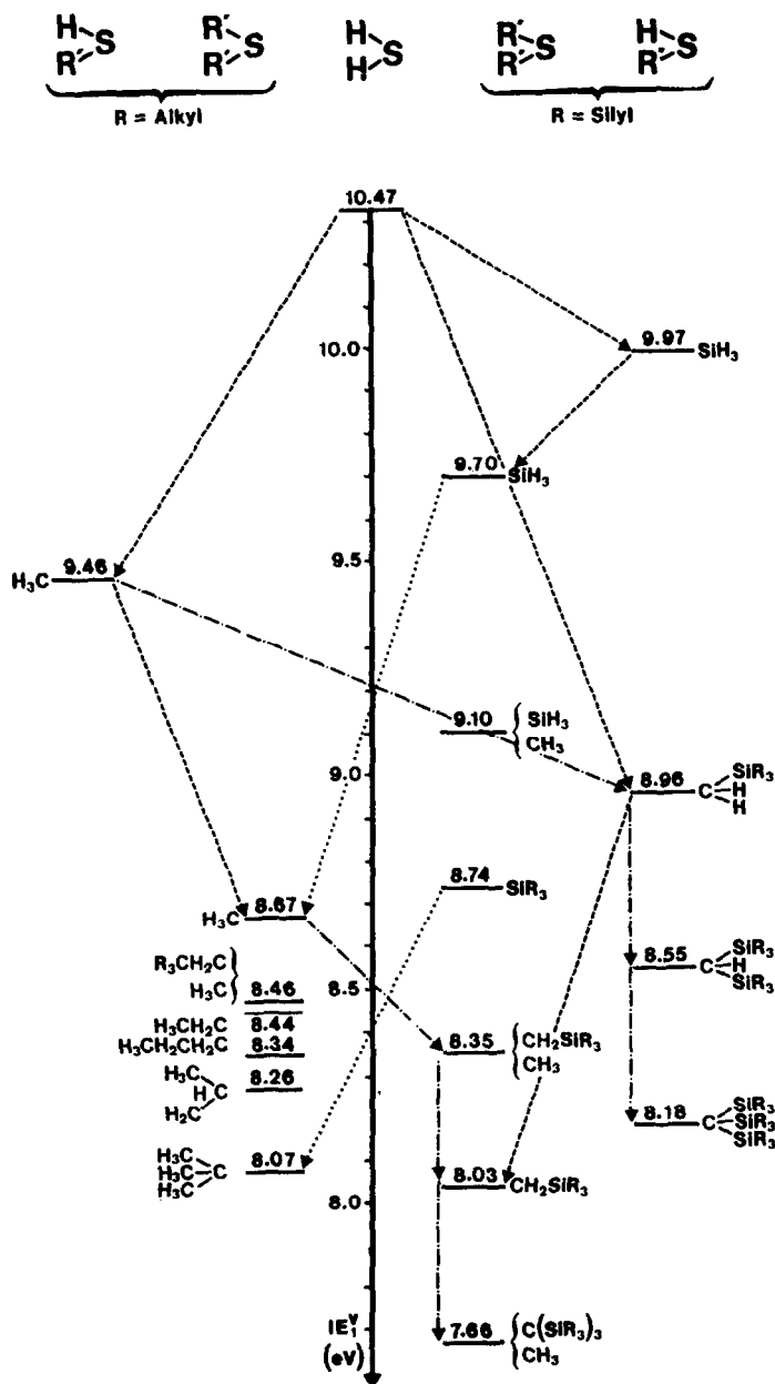
Fig. 2. First vertical ionization energies of \text{H}_2\text{S} and its alkyl, silyl, trimethylsilyl and trimethylsilylmethyl derivatives (connecting lines: ----- identical mono- and di-substitution; ..... alkyl/silyl comparison; -.-.- \beta silyl substituent effects).
