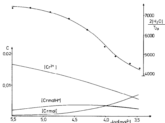
Fig. 2. Concentration distribution of the complexes formed in the Cr 2+ -malonic acid system, together with the change of the relaxation rate of water protons, as a function of free malonate concentration.
