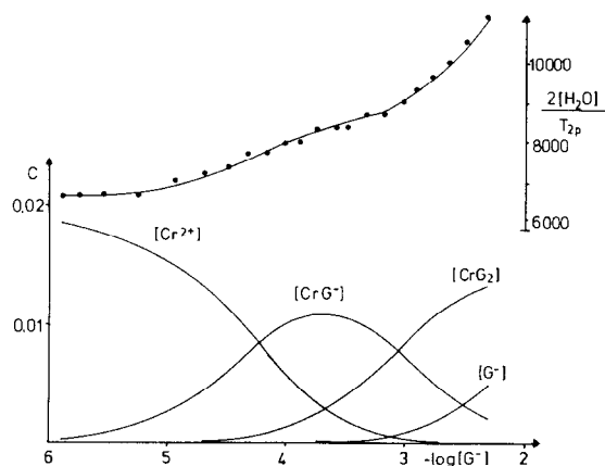
Fig. 1. Concentration distribution of the complexes formed in the Cr 2+ -glycine system, together with the change of the relaxation rate of water protons as a function of free glycinate concentration.
