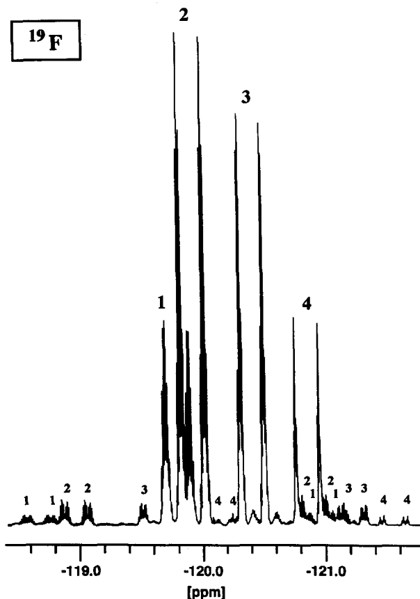
Fig. 1. ^{19}\text{F} NMR spectrum of the \text{CF}_2\text{H} part of (\text{CF}_3)_n(\text{CF}_2\text{H})_{4-n}\text{Sn} . The main signals and their ^{119}/^{117}\text{Sn} satellites are denoted by the number, n , of \text{CF}_2\text{H} groups.
