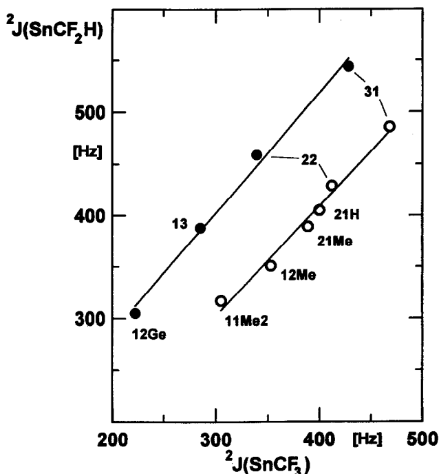
Fig. 2. Correlation of the ^2J(\text{SnF}) coupling constants of \text{SnCF}_2\text{H} and \text{SnCF}_3 groups in mixed (trifluoromethyl)(difluoromethyl)stannanes, (\text{CF}_3)_n(\text{CF}_2\text{H})_m\text{SnR}_{4-n-m} . The digits in the figure give the values of n and m , and the R groups are designated explicitly ( \text{Ge} \triangleq \text{GeMe}_3 ). Solid circles (●) refer to solutions containing fluoride ( \text{GeMe}_3\text{F} ).
