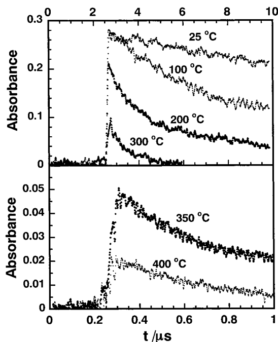
Figure 1. Temporal profiles of (\text{SCN})_2^{\bullet-} in 0.01 m KSCN solution, \text{N}_2\text{O} -saturated, dose = 35 Gy pulse -1 . Conditions: 25–200 °C, 200 atm; 300 °C, 250 atm; 350 °C, 300 atm; 400 °C, 350 atm.
