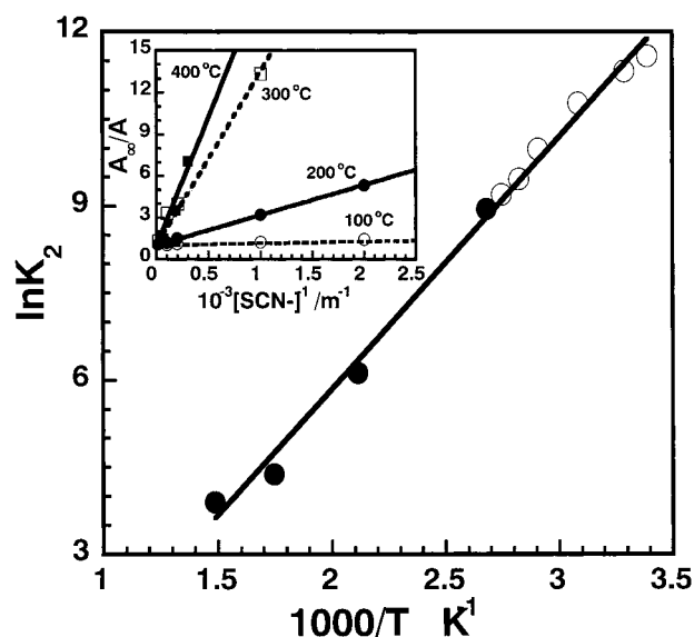
Figure 5. Van't Hoff plot of K_2 over 15–90 °C (O, Elliot et al. 13 ) and 100–400 °C (●, this work). Water densities are 0.967 (100 °C), 0.878 (200 °C), 0.743 (300 °C), and 0.475 (400 °C) g/cm 3 . Inset: Plots of A_\infty/A as a function of [\text{SCN}^-] for (\text{SCN})_2^{*-} at various temperatures.
