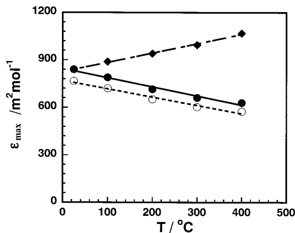
Figure 8. Molar absorption coefficient of (\text{SCN})_2^{\bullet-} as a function of temperature: (●) using the G(\text{e}_{\text{aq}}^-) and G(\text{OH}^\bullet) values shown in Table 2; (○) calibrated using G(\text{OH}^\bullet) = 0.63 \mu\text{mol/J} at room temperature in \text{N}_2\text{O} -saturated KSCN solution as compared to G(\text{e}_{\text{aq}}^-) + G(\text{OH}^\bullet) = 0.57 \mu\text{mol/J} but assuming the same temperature dependence as shown in Table 2; (◆) assuming the temperature independence of G values.
