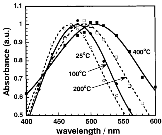
Figure 2. Normalized absorption spectra of (\text{SCN})_2^{\bullet-} at different temperatures. Conditions: [KSCN] = 0.01 m; 25–200 °C, 200 atm; 400 °C, 350 atm.
