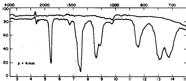
Figure 3.—Infrared spectrum of \text{SF}_2=\text{NCOF} .
