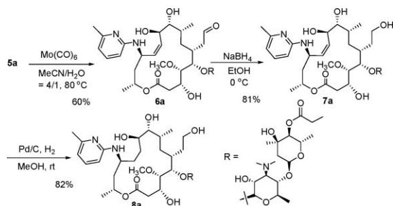
Scheme 1 Chemical modification of leucomycin adduct 5a .
