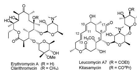
Fig. 1 Structures of representative 14- and 16-membered macrolides.
