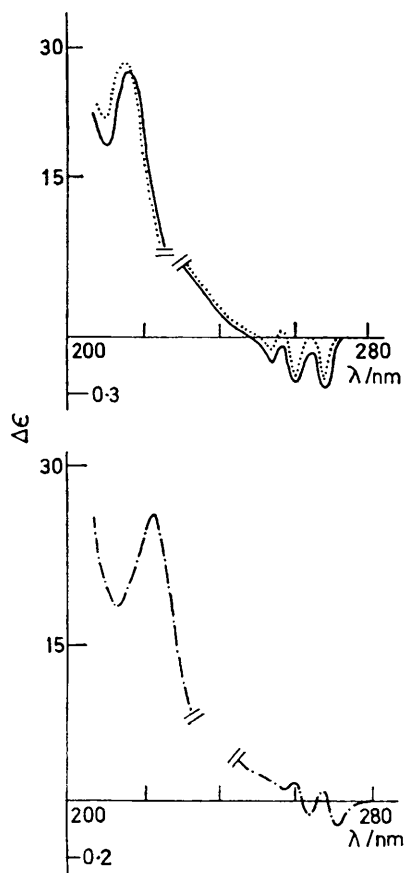
C.d. curves of oxadiazoles (Va) (— · — · —) ( \lambda_{\text{max}} , 275inf., 272, 263, 257, 252, and 220 nm); (Vb) (· · · · ·) ( \lambda_{\text{max}} , 266inf., 263, 257, 251, 248, and 220 nm); (Vc) (—) ( \lambda_{\text{max}} , 267inf., 263, 257, 251, 247, and 218 nm)
