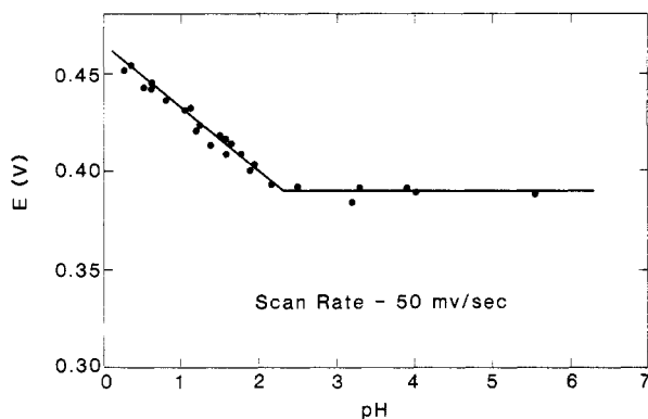
Figure 2. Acid dependence of E for the [(\text{NH}_3)_5\text{Ru}_2(\text{MN})] complex as measured by cyclic voltammetry.
