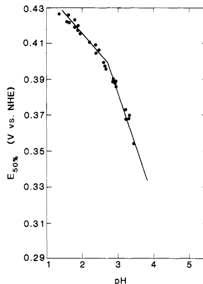
Figure 3. Acid dependence of the potential at 50% oxidation for the [(\text{NH}_3)_5\text{Ru}_2(\text{MN})] complex.
