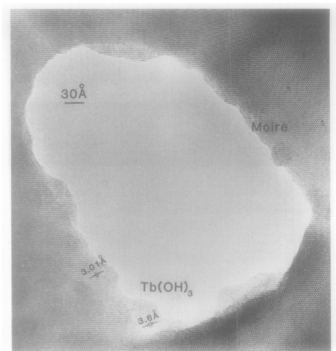
FIG. 12. A high-resolution image of the region of the leached hole of Fig. 10. Notice the moiré pattern at the right, the disordered projection at the bottom, and the region marked \text{Tb(OH)}_3 with considerable order, each suggesting incomplete oxidation.
