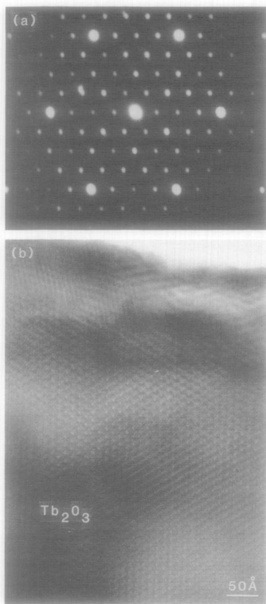
FIG. 8. A diffraction pattern (a) and the image (b) showing that, in the process of solvolytic disproportionation, regions of C-type \text{Tb}_2\text{O}_3 are formed prior to their dissolution.
