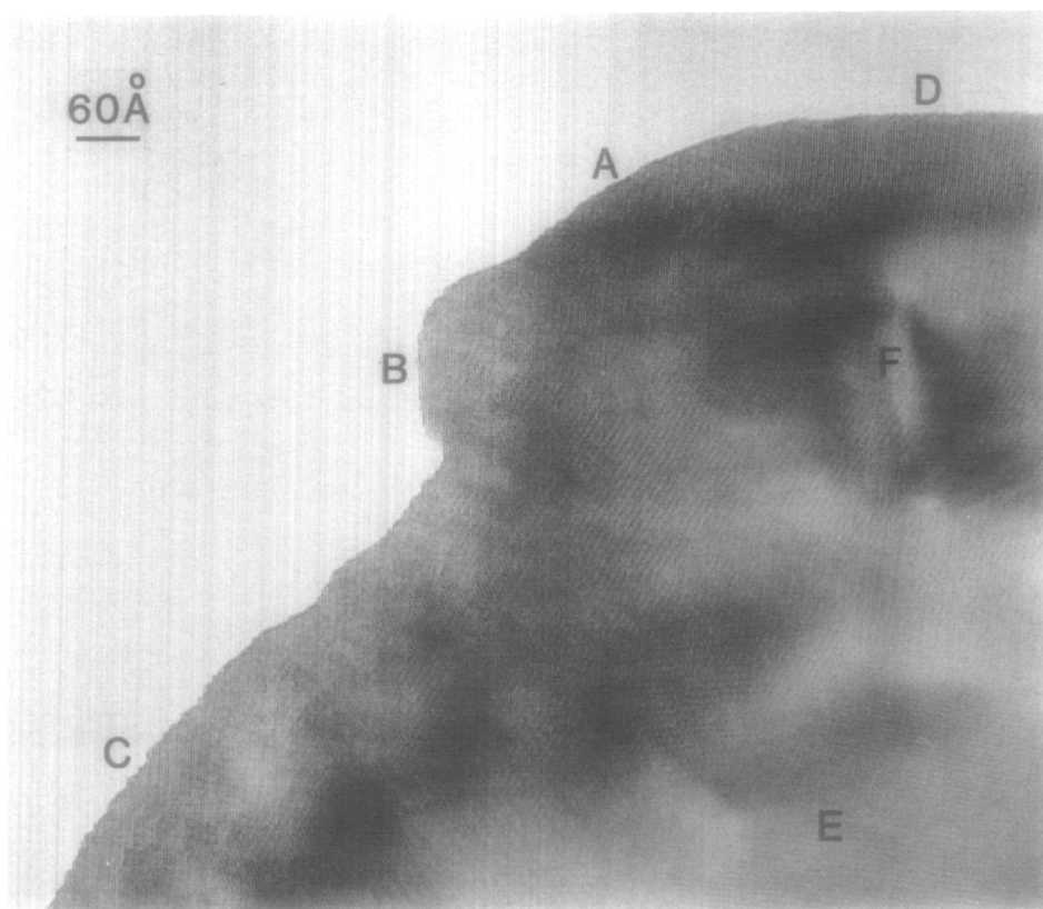
FIG. 3. A high-resolution image of the \text{TbO}_x starting material. The various surfaces and their morphology are labeled A, B, C, and D. Two dislocations are marked E and F.
