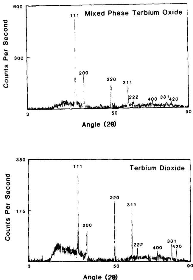
FIG. 2. A powder X-ray diffraction pattern of \text{TbO}_x (top). The broadened lines result from the two-phased mixture of \text{Tb}_7\text{O}_{12} and \text{Tb}_{11}\text{O}_{20} . A powder X-ray diffraction pattern of the product \text{TbO}_2 is at the bottom.
