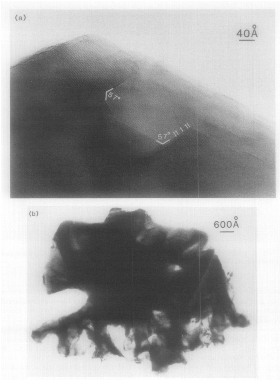
FIG. 4. The morphology of chemically leached \text{TbO}_x . (a) A leach pit developed with \{111\} walls in the early stages of reaction. (b) The final product consisting of a network of \text{TbO}_2 material enclosing fully developed leach pits.
