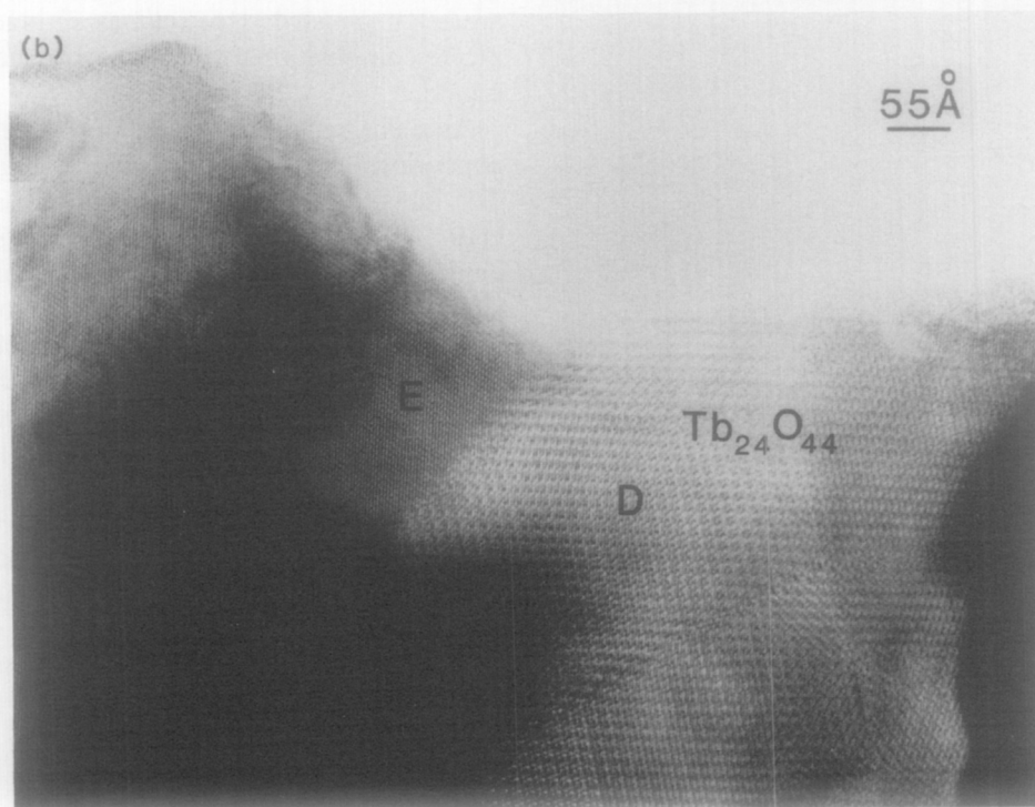
FIG. 9. High-resolution images of an oxidized intermediate phase formed during solvolytic disproportionation. (a) Three regions are marked A, B, and C where three orientational variants of \text{Tb}_{24}\text{O}_{44} exist having 3-, 4- and 8-metal atom columns in the projected unit cell, respectively. (b) An image of domains of \text{Tb}_{24}\text{O}_{44} in the [21\bar{1}] zone, D, and the orientational variant, E, that is an inversion of that marked A in (a).
