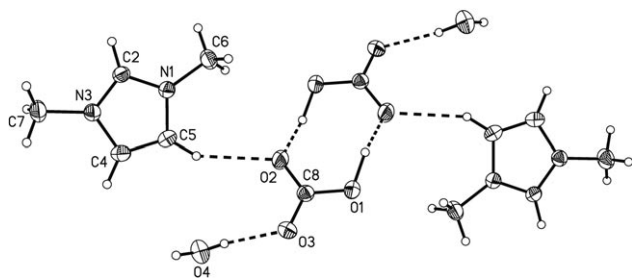
Figure 2. ORTEP illustration (50% probability thermal ellipsoids) of the [1,3\text{-diMIM}][\text{HCO}_3]\cdot\text{H}_2\text{O} hydrogen-bonded dimer.
