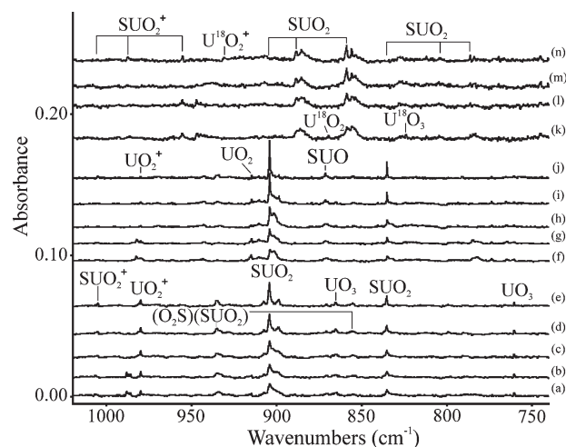
Figure 3. Infrared spectra in the 1020–740 \text{cm}^{-1} region for products formed in the laser-ablated uranium atom reaction with sulfur dioxide during condensation in excess neon at 5 K. (a) Normal isotopic ^{32}\text{SO}_2 isotopic sample at 0.2% in argon co-deposited for 60 min, (b) after annealing to 8 K, (c) after >220 nm irradiation, (d) after annealing to 10 K, (e) after annealing to 12 K, (f) ^{34}\text{SO}_2 isotopic sample at 0.2% in argon co-deposited, (g) after annealing to 8 K, (h) after >220 nm irradiation, (i) after annealing to 10 K, (j) after annealing to 12 K, (k) \text{S}^{18}\text{O}_2 and \text{S}^{16,18}\text{O}_2 isotopic mixture at 0.1% co-deposited, (l) after annealing to 8 K, (m) after annealing to 10 K, (n) after annealing to 12 K.
