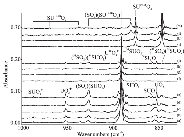
Figure 2. Infrared spectra in the 1000–830 \text{cm}^{-1} region for products formed in the laser-ablated uranium atom reaction with sulfur dioxide during condensation in excess argon at 5 K. Expanded absorbance scale for the same spectra presented in Figure 1.
