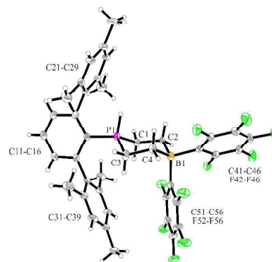
Figure 1. A view of the molecular structure of the P/B/B hydrogenation product 14a (thermal ellipsoids are shown with 50 % probability). Selected bond lengths (Å) and angles (°): P1-C1 1.786(3), P1-C3 1.786(3), C1-C2 1.540(4), C3-C4 1.546(5), C2-B1 1.648(5), C4-B1 1.652(5), C1-P1-C3 106.7(2), C2-B1-C4 107.5(3), \Sigma \text{P1}^{\text{CCC}} 339.2(5).
