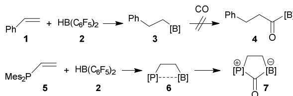
[B]: B(C 6 F 5 ) 2 ; [P]: PMes 2 Scheme 1. Behavior of strongly electrophilic pentafluorophenyl containing boranes toward carbon monoxide.
