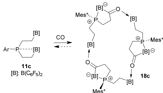
Scheme 5. Formation of the cyclotrimeric carbonylation product 18c .
