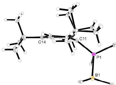
Figure 4. Side view of a 2,4,6-tri- t -butylphenyl-P (i.e. Mes*-P) unit of the macrocyclic trimer 18c . The P1-C11-C14 angle of this unit amounts to 144.1°.
