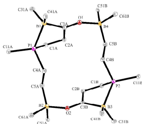
Figure 2. A view of the structure of the framework of macrocyclic dimer 17b (the bulky substituents at boron and phosphorus were omitted for clarity; thermal ellipsoids are shown with 50 % probability). Selected bond lengths (Å) and angles (°): P1-B1 2.063(2), B1-C3A 1.632(3), C3A-O1 1.254(2), O1-B4 1.609(2), P2-B3 2.067(2), B3-C3B 1.648(3), C3B-O2 1.255(2), O2-B2 1.618(2), B1-C3A-O1 120.8(2), C3A-O1-B4 129.6(1), B3-C3B-O2 122.7(2), C3B-O2-B2 130.8(1).
