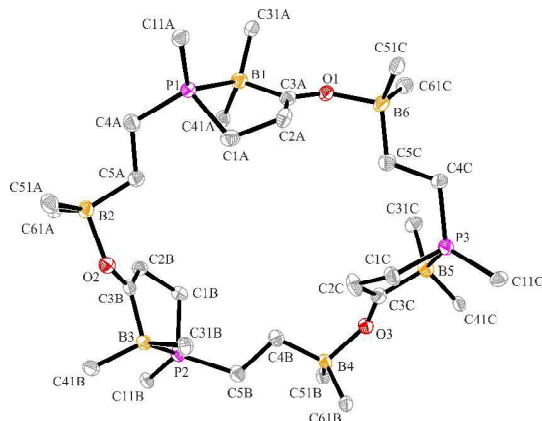
Figure 3. A view of the core structure of the macrocyclic P/B/B carbonylation trimer 18c (the substituents at boron and phosphorus are omitted for clarity; thermal ellipsoids are shown with 15 % probability). Selected bond lengths (Å) and angles (°) of the molecular: P1-B1 2.096(5), C3A-O1 1.253(5), O1-B6 1.590(6), P3-B5 2.110(5), C3C-O3 1.245(5), O3-B4 1.603(6), P2-B3 2.094(5), C3B-O2 1.239(5), O2-B2 1.625(6), B1-C3A-O1 117.7(4), C3A-O1-B6 133.7(3), B5-C3C-O3 119.6(4), C3C-O3-B4 133.4(3), B3-C3B-O2 118.3(4), C3B-O2-B2 131.9(4).
