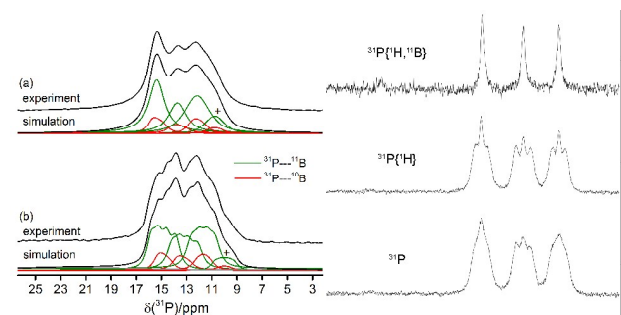
Figure 5. 31 P MAS NMR spectra obtained for the C_1 -symmetric macrocyclic trimer 18c . Left: (a) 31 P{ 1 H} CP/MAS NMR spectrum of 18c with 1 H and 11 B decoupling, (b) 31 P MAS NMR spectrum with 1 H decoupling only and corresponding simulations, based on the indirect 31 P- 11 B and/or 31 P- 10 B spin-spin interactions. The symbol + marks a suspected impurity. Right: 31 P, 31 P{ 1 H}, and 31 P{ 1 H, 11 B} NMR spectra of compound 18c in solution (CD 2 Cl 2 , 203 K).
