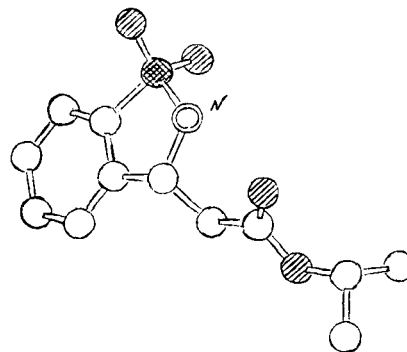
Figure 4—X-Ray crystallographic sketch of Compd. III.
