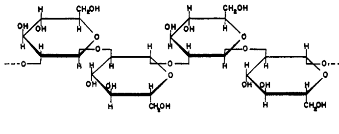
Fig. 1.—Arrangement of the \beta -glucose residues joined through 1,2-glucosidic linkages
