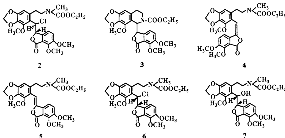
Chart 1. Degradation Products Obtained from \alpha -Narcotine ( 1 ) with Excess ECF under Reflux
