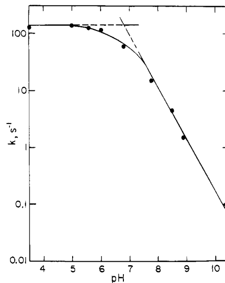
Figure 2. Observed rate constant of the formation of I_3^- in the oxidation of I^- by peroxynitrite as a function of pH. Solutions contained 6 mM iodide, 0.33 mM peroxynitrite, and 0.1 M phosphate.
