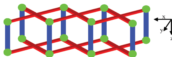
Figure 1. Cartoon representation of the 2D sheet formation by the tetraacid ligand (red) pillared by a dipyrrolic strut (blue). The green corners are the zinc paddlewheel nodes.
