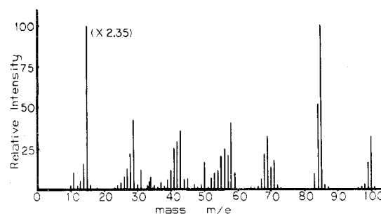
Figure 3. Mass spectrum of (\text{CH}_3)_2\text{B}_2\text{O}_3 .
