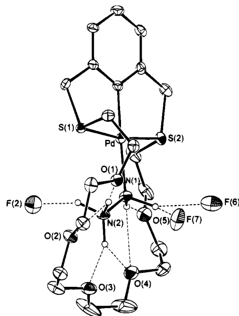
Figure 10. Alternative view of the [\text{Pd}(\text{L}^5)(\text{NH}_2\text{NH}_3)]^{2+} cation emphasizing the orientation of the polyether ring to the substrate and showing the substrate interactions with F(2) of one \text{BF}_4^- anion and F(6) and F(7) of the other.
