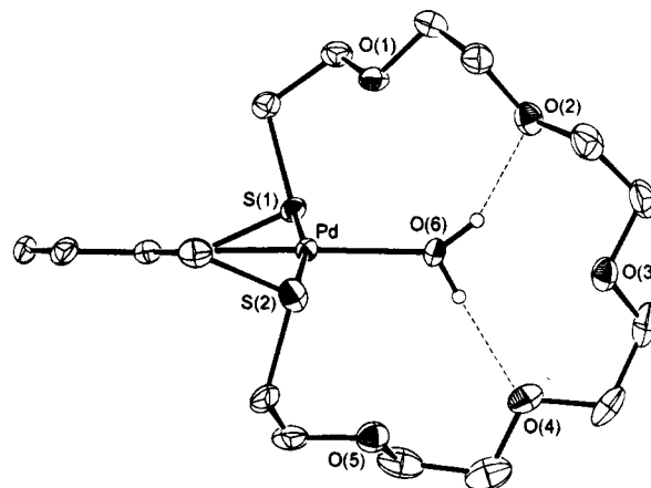
Figure 4. Alternative view of the [Pd(L 5 )(H 2 O)] + cation emphasizing the orientation of the polyether ring to the substrate.
