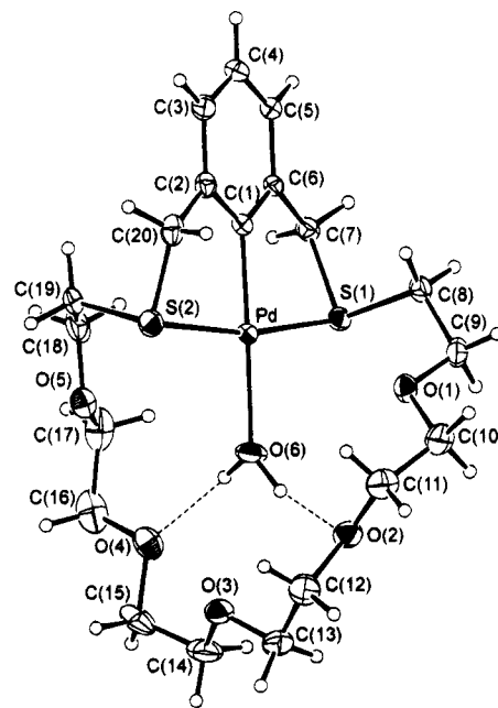
Figure 3. Structure of the [\text{Pd}(\text{L}^5)(\text{H}_2\text{O})]^+ cation showing the atom-numbering scheme and hydrogen-bonds to the metalloreceptor.
