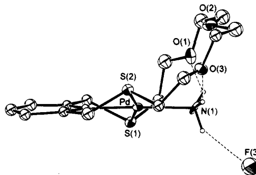
Figure 2. Alternative view of the [\text{Pd}(\text{L}^3)(\text{NH}_3)]^+ cation emphasizing the orientation of the polyether ring to the substrate and showing the substrate interaction with F(3) of the \text{BF}_4^- anion.
