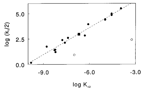
Figure 3. LFER for the second-order path of oxidation reactions of I^- . The oxidants are as follows: \text{Fe}(\text{phen})_3^{3+} , \text{Fe}(5,6-(\text{CH}_3)_2\text{-phen})_3^{3+} , \text{Fe}(4,7-(\text{CH}_3)_2\text{-phen})_3^{3+} , \text{Fe}(3,4,7,8-(\text{CH}_3)_4\text{-phen})_3^{3+} , \text{Fe}(\text{bpy})_3^{3+} , \text{Fe}(4,4'-(\text{CH}_3)_2\text{-bpy})_3^{3+} , \text{IrCl}_6^{2-} , \text{IrBr}_6^{2-} , \text{Mo}(\text{CN})_8^{2-} , \text{Os}(\text{bpy})_3^{3+} , \text{Os}(\text{phen})_3^{3+} (●); \text{ClO}_2 (■); \text{NpO}_2^{2+} , \text{PuO}_2^{2+} (○). The data were used as given or cited in refs 13–15.
