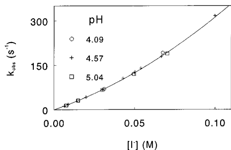
Figure 1. The pseudo-first-order rate constant as a function of iodide concentration at various pH values (25.0 °C, I = 1.0 M NaClO 4 ).
