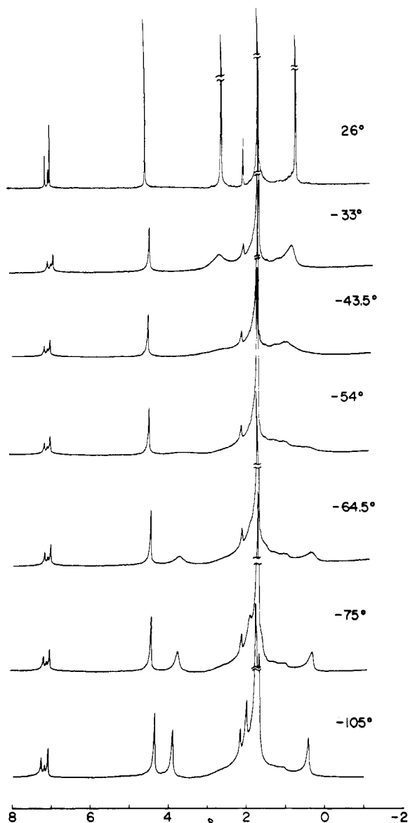
Figure 1. Variable-temperature ^1\text{H} NMR spectra of bis(2,4-dimethylpentadienyl)ruthenium in \text{toluene-}d_8 . A resonance at ca. 2.3 ppm and the resonances around 7.3 ppm are due to the solvent.
