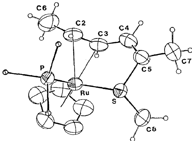
Fig. 2. An ORTEP-drawing of [CpRu(PPh 2 Me)(η 3 -S(Me)C(Me)=CHCH=CH(Me))]BF 4 (9d).
