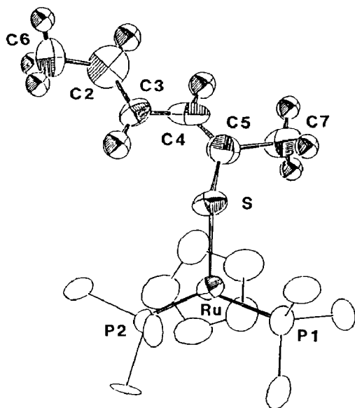
Fig. 1. An ORTEP-drawing of [CpRu(PPh 2 Me) 2 (η 1 -SC(Me)=CHCH=CH(Me))] (6d).
