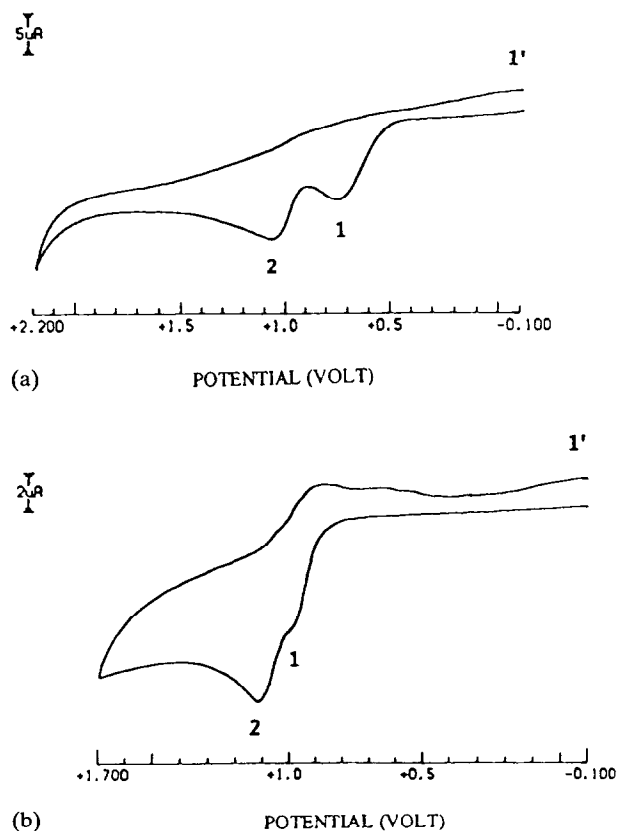
Fig. 4. (a) Cyclic voltammogram of a 2.0 mM solution of [Rh 2 (ox)(COD) 2 ] in CH 3 CN, 0.20 M TBAP. Scan rate of 100 mV/s. (b) Cyclic voltammogram of a 2.0 mM solution of [Rh 2 (ox)(COD) 2 ] in CH 2 Cl 2 , 0.20 M TBAP. Scan rate of 100 mV/s.
