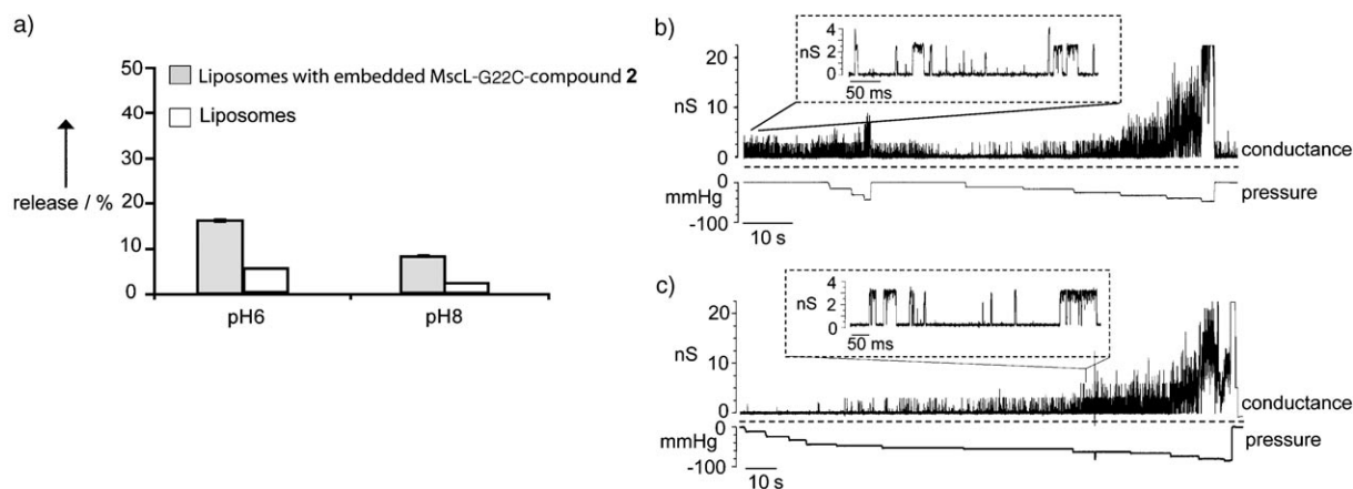
Figure 2. Activity of MscL-G22C modified with 2 . Modified MscL was reconstituted in 1,2-dioleoyl- sn -glycero-3-phosphocholine (DOPC) liposomes at a protein/lipid ratio of 1:120 (wt/wt) with a detergent-mediated reconstitution method. The fluorescent dye calcein (final concentration 50 mM) was added to the lipid–protein mixture and the detergent was removed with biobeads. External calcein was removed by column chromatography on Sephadex G50 and the liposomal fraction was used in the efflux assay. Depending on the concentration, about 10 \mu L of liposomes were diluted in 2 mL isoosmotic buffer (330 mosm) with varying pH values, and the increase in fluorescence was monitored for 45 min. Maximum release was reached within 30 min and is reported here relative to the release obtained after bursting the liposomes with excess Triton X100. Error bars indicate the standard deviation of two separate experiments. a) pH-induced release in calcein efflux assays. At pH 8, the proteoliposomes released about 8% of the dye, but at pH 6 the release increased to 16%. Patch-clamp measurements at b) pH 5.8 and c) at pH 8. Insets: typical channel openings in an enlarged form. The channel opened spontaneously without applied tension at pH 5.8. The observed conductance was about 2.5 nS, but if tension was applied gradually, the channel also gated to its full conductance of 3 nS with as little as 15 mmHg applied negative pressure. Conversely, at pH 8 spontaneous gating was absent and only the tension-dependent openings were observed. At lower tensions (up to –50 mmHg pressure in the patch) the channel opened to lower subconducting states (1 and 2 nS), whereas at higher levels of applied tension the full conductance was reached. Further application of tension resulted in the opening of more than one channel.
