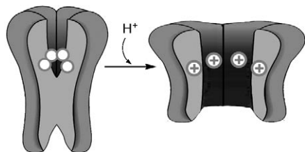
Figure 1. Protonation-induced opening of a mechanosensitive channel, which shows four of the five subunits in the pentamer (conceptual drawing). Protonation of a hydrophobic pore region of the MscL results in conformational changes and channel opening.
