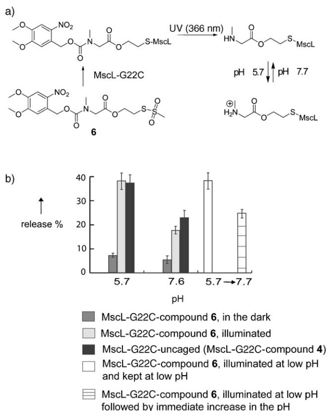
Figure 4. MscL-G22C modified with a caged pH modulator. a) Structure of 6 and removal of the protecting group by illumination. b) Activity of the modified MscL-G22C channels in the efflux assay. Channels modified with caged modulator 6 did not open at any pH value in the dark (dark gray bars). After deprotection by irradiation at 366 nm for 10 min (spectroline long-life filter, 365 mWcm -2 ), channels became activated and released the liposomal content in dependence on the ambient pH (light gray bars). If the pH of the protein sample, which was illuminated at low pH, was immediately raised to 7.7 ± 0.1, the release of dye stopped (white bar with horizontal lines) because of closing of the channel; if the pH was kept constant at a low value, the channel stayed open (white bar) and release continued. Channels modified with uncaged modulator 4 opened in response to pH (black bar). Error bars indicate the standard deviation from three independent experiments.
