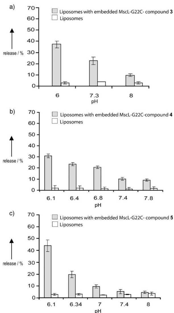
Figure 3. pH-dependent activity of modified MscL in calcein efflux assays. Modified MscL was reconstituted in DOPC/cholesterol/DSPE-PEG2000 (70:20:10 m) liposomes in the presence of calcein. The activity of the channel at different pH values was monitored to determine the maximum release values. Release was invariably completed within 30 min. Error bars indicate the standard deviation from four independent experiments. MscL-G22C modified with a) 3 , b) 4 , and c) 5 . DSPE=1,2-distearoyl- sn -glycero-3-phosphoethanolamine; PEG= polyethylene glycol.
