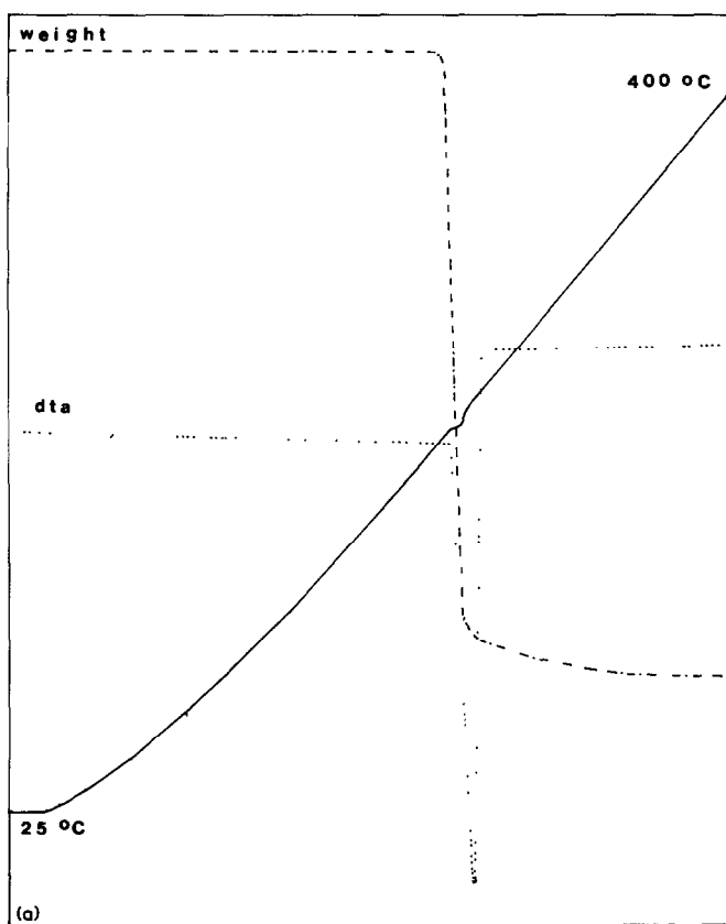
Fig. 1. TGA (---) and DTA (.....) curves for (a) \text{Cu(nic)}_2 and (b) \text{Cu(isonic)}_2 \cdot 4\text{H}_2\text{O} . Linear heating is also shown (—).
