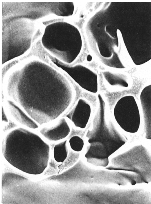
Fig. 2. SEM picture of the pyrolysis (400 °C) product of Cu(nic) 2 .
