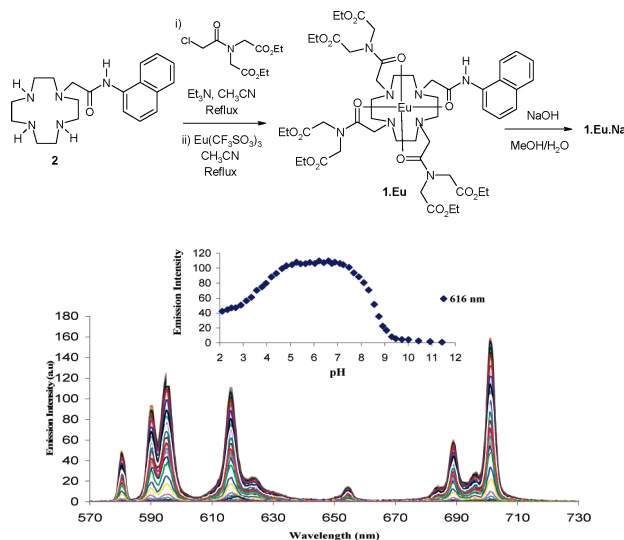
Figure 1. Changes in the Eu(III) luminescence of 1.Eu.Na upon excitation of the naphthalene antenna as a function of pH ( I = 0.1 M NEt 4 HClO 4 (TEAP)). Insert: The changes at 616 nm vs pH.
