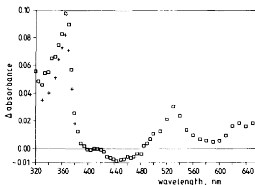
Fig. 4. Spectrum (□) obtained 1 \mu\text{s} after a 266 nm laser pulse delivered to an aqueous solution of 3.32 \times 10^{-4} M \text{K}_2[\text{Fe}(\text{bpy})(\text{CN})_4] and 1 M KCl; spectrum (+) taken 1 \mu\text{s} after an electron pulse is delivered to 2 \times 10^{-4} M \text{K}_2[\text{Fe}(\text{bpy})(\text{CN})_4] in water containing 2% tert-butyl alcohol.
