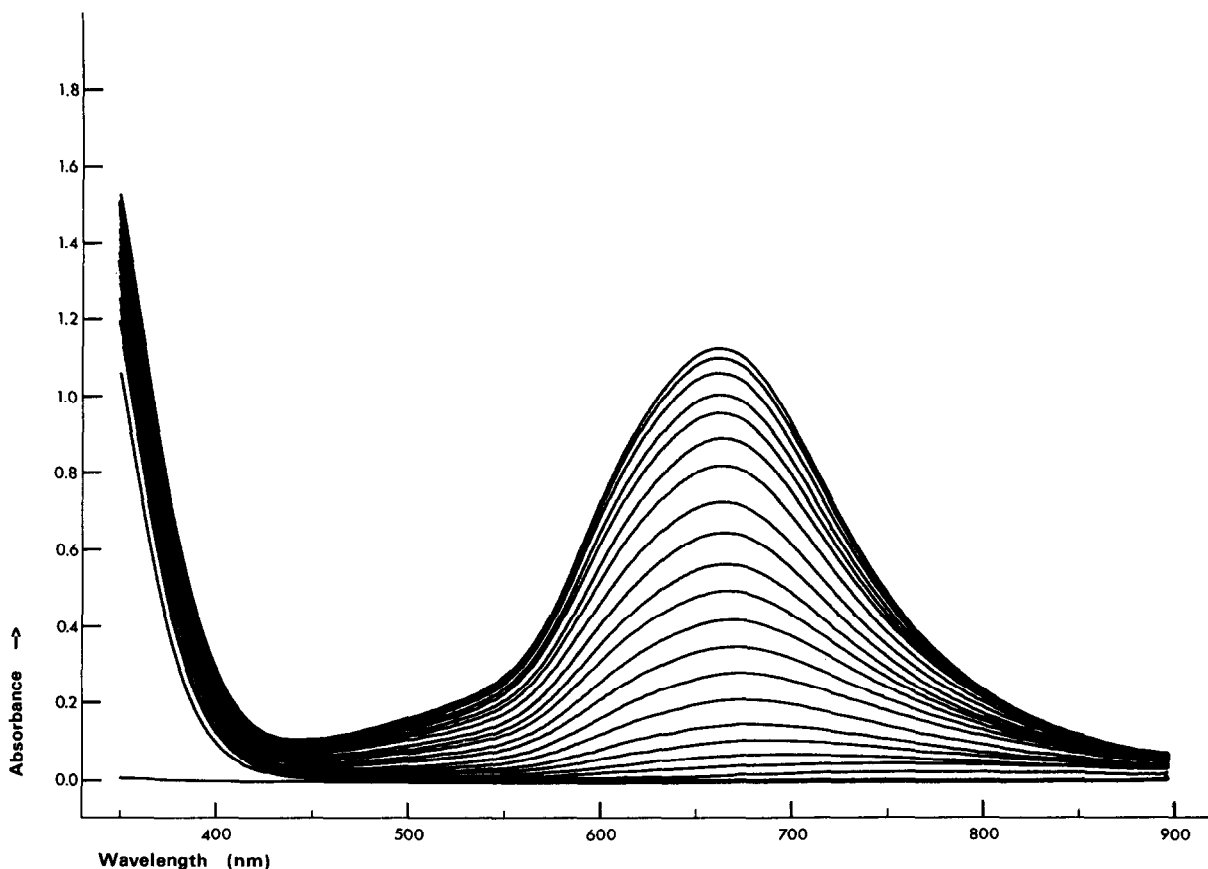
Fig. 1. Visible spectra at 20 minute intervals of a solution initially 0.44 M in each of \text{cis-}[\text{Pt}(\text{NH}_3)_2(\text{H}_2\text{O})_2](\text{NO}_3)_2 and \text{KH}_2\text{PO}_4 , adjusted to pH 3.0 (small amounts of solid filtered off).
