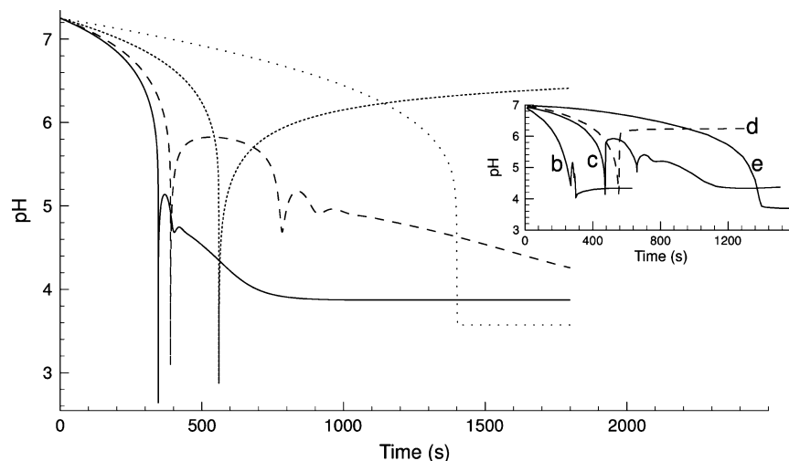
Figure 6. Calculated pH–time curves on the basis of model (M1)–(M4) in batch condition. Conditions: [S_2O_3^{2-}]_0 = 0.011 M; [HSO_3^-]_0 + [SO_3^{2-}]_0 = 0.0195 M; [H^+]_0 = 0.007 M; [IO_3^-]_0/M = 0.0125 (solid line), 0.0115 (long dashed line), 0.009 (short dashed line), 0.0055 (dotted line). The inset, which was taken from a part of Figure 1 of the original Rábai and Beck paper, 14 shows the measured pH–time curves as the iodate concentration changes.
