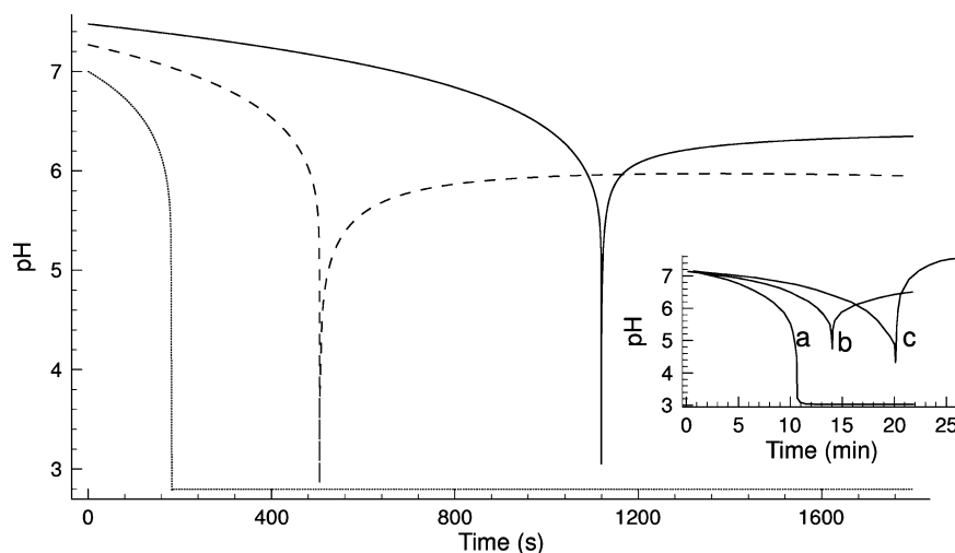
Figure 5. Calculated pH–time curves on the basis of model (M1)–(M4) in batch condition. Conditions: [S_2O_3^{2-}]_0 = 0.01 M; [IO_3^-]_0 = 0.01 M; [HSO_3^-]_0 + [SO_3^{2-}]_0 = 0.02 M; [H^+]_0/M = 0.005 (solid line), 0.007 (dashed line), 0.01 (dotted line). The inset, which was taken from a part of Figure 1 of the original Rábai and Beck paper, 24 shows the measured pH–time curves as [H^+]_0 changes.
