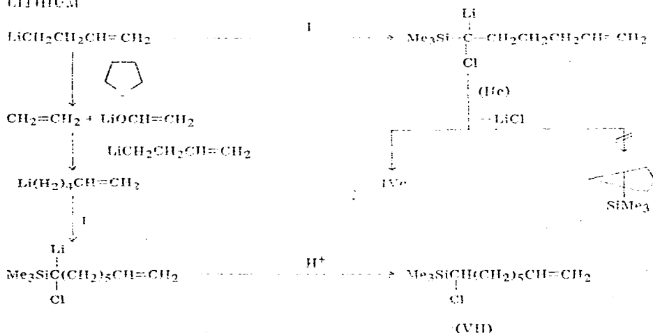
SCHEME 3. THE REACTION OF c -CHLOROVINYLTRIMETHYLSILANE WITH 3-BUTENYL-LITHIUM
