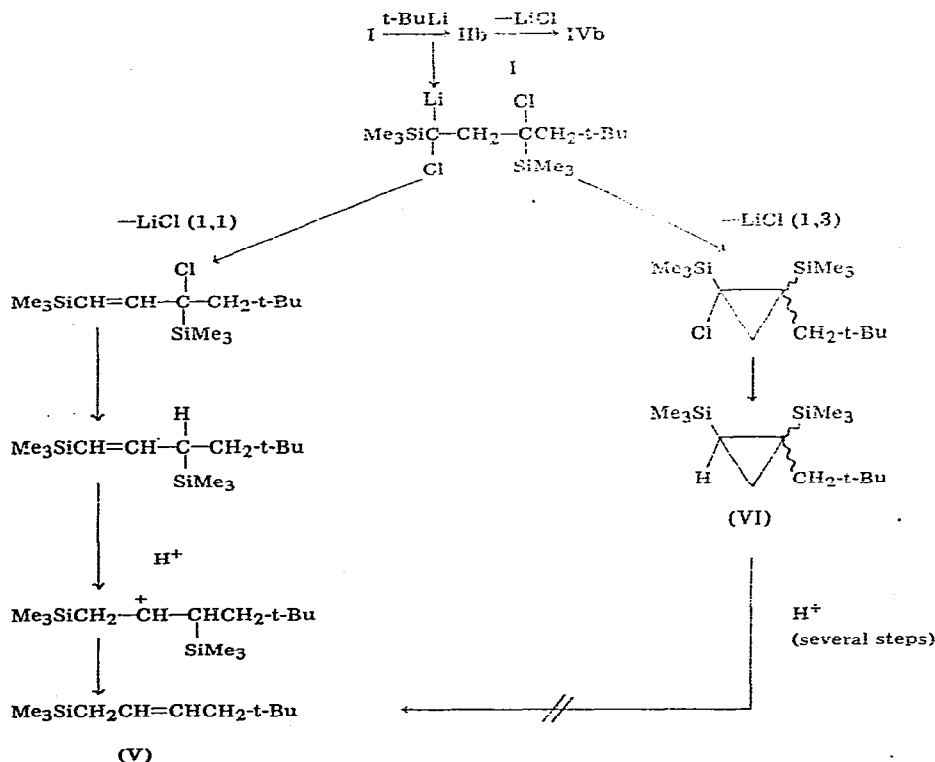
SCHEME 2. POSSIBLE BEHAVIOR OF THE SYSTEM \alpha -CHLOROVINYLTRIMETHYLSILANE/ t -BUTYLLITHIUM AT -78^\circ\text{C}
