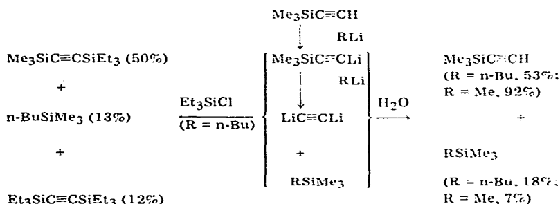
SCHEME 4. REACTION OF ETHYNYLTRIMETHYLSILANE WITH ALKYL LITHIUM REAGENTS
