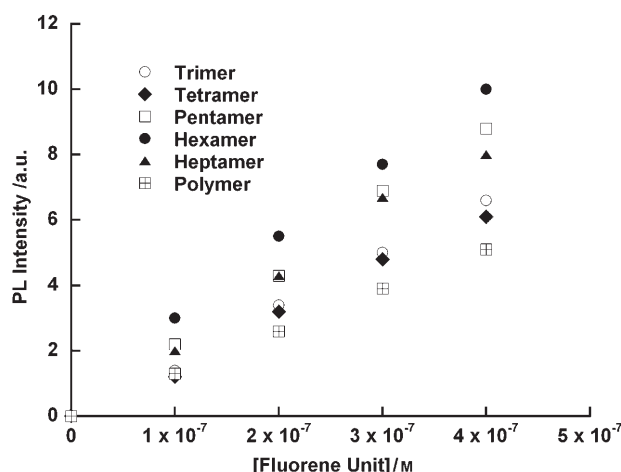
Figure 5. Fluorescence intensity of the donor-sensitized dsDNA-FI emission with varying oligomer/polymer concentrations based on fluorene units. [dsDNA] = 2 \times 10^{-8} M.
