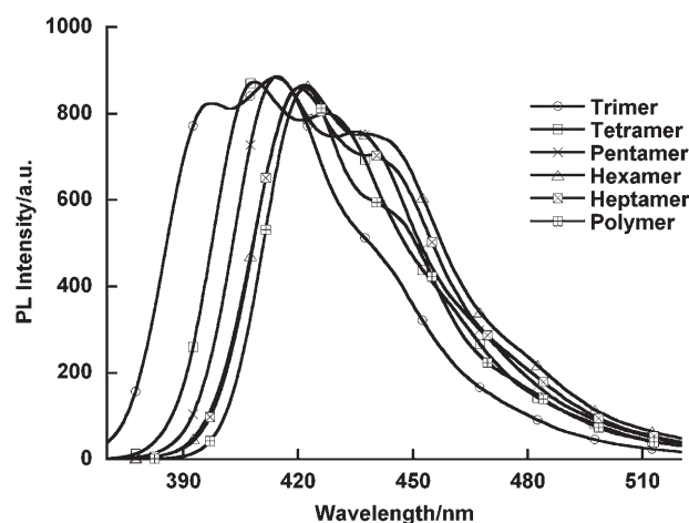
Figure 3. The emission spectra of the fluorenyl oligomers 16–20 and the polymer in water at [fluorene unit] = 3.0 \times 10^{-6} \text{ M} .
