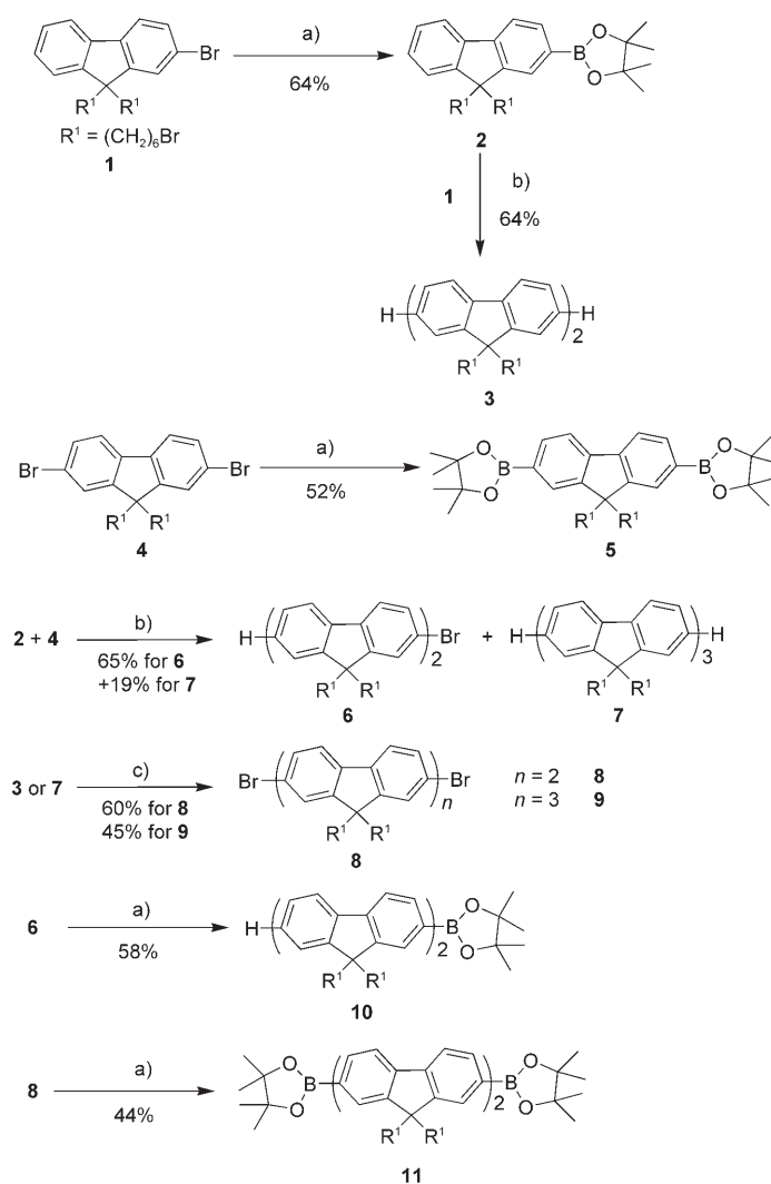
Scheme 1. Synthetic route to the intermediates for the oligomers. a) bis-(pinacolato)diboron, [PdCl 2 (dppf)], KOAc, dioxane, 80 °C; b) [Pd-(PPh 3 ) 4 ], 2 M K 2 CO 3 , toluene/H 2 O, 100 °C; c) Br 2 /I 2 , dichloromethane. dppf = 1,1'-bis(diphenylphosphino)ferrocene.
