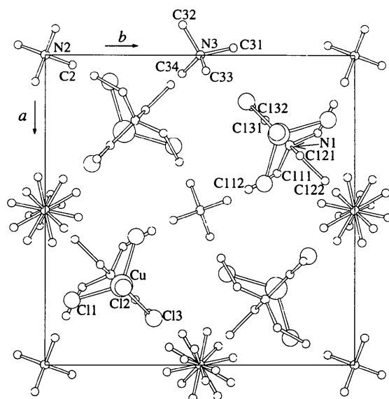
Fig. 1. An ORTEP (Johnson, 1976; André & Michalowicz, 1991) drawing with atomic labelling scheme viewed along [001]. Atoms are drawn as spheres of arbitrary radii. Only one position of the disordered TMA cation at (0, \frac{1}{2} , 0.0054) is shown.
