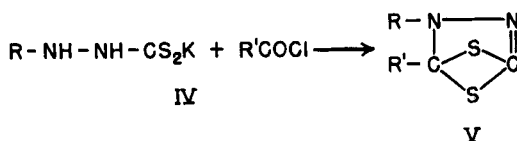
Scheme II
