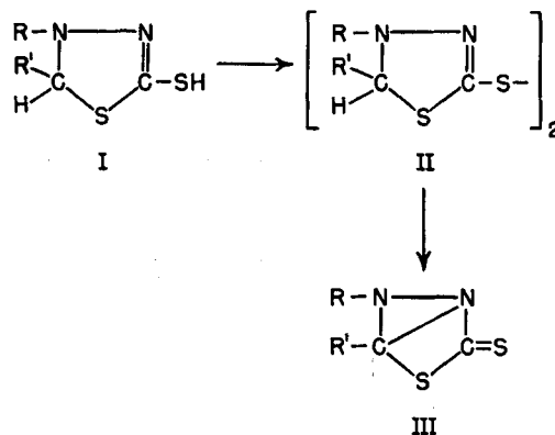
Scheme I
