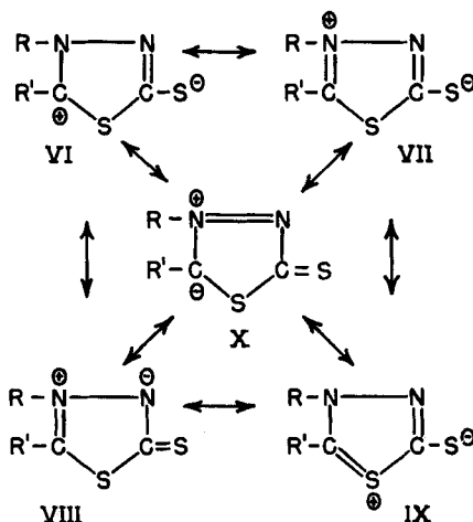
Scheme III
