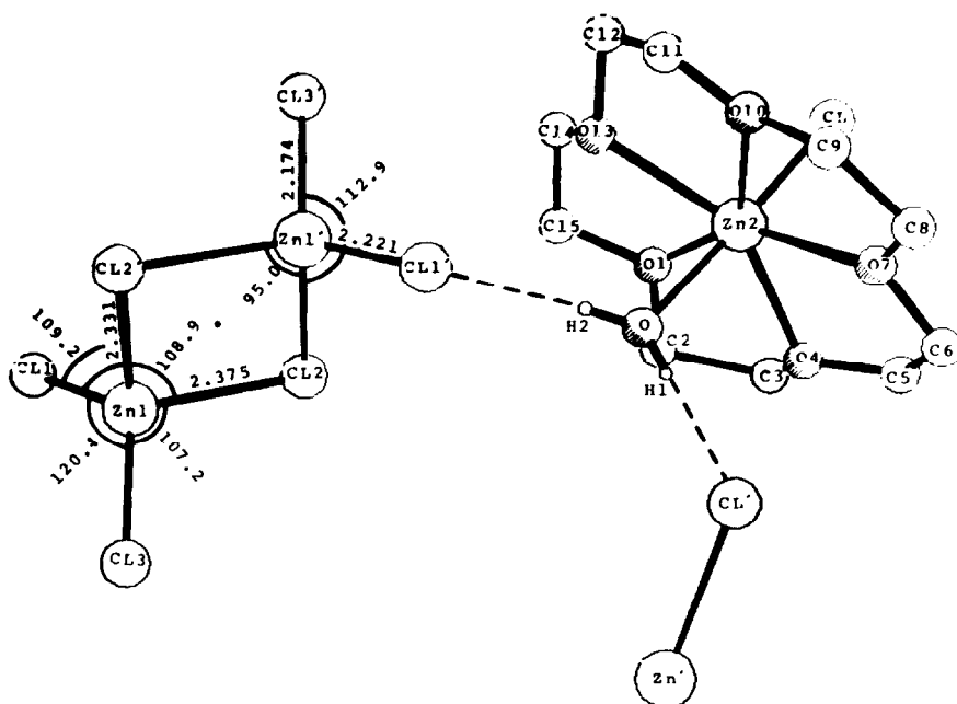
Fig. 2. The structure of the complex salt [\text{ZnCl} \cdot 15\text{-crown-5} \cdot \text{H}_2\text{O}]_2^{2+}[\text{Zn}_2\text{Cl}_6]^{2-} (III).
