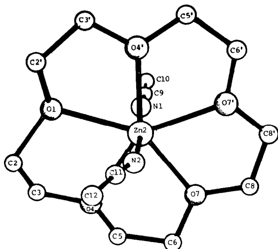
Fig. 1. The structure of the cation [\text{Zn} \cdot 15\text{-crown-5} \cdot 2\text{CH}_3\text{CN}]^{2+} in the complex [\text{Zn} \cdot 15\text{-crown-5} \cdot 2\text{CH}_3\text{CN}]^{2+}[\text{Zn}_2\text{Cl}_6]^{2-} \cdot \text{CH}_3\text{CN} (II). (The H atoms of the crown-ether molecules are omitted for clarity in this and all following Figures.)
