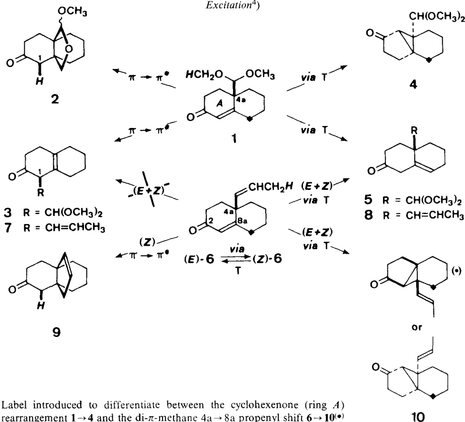
Scheme 1. Photochemical Transformations of 4a-Dimethoxymethyl-bicyclo[4.4.0]dec-1(8a)-en-2-one ( 1 ) [2] and the 4a-(1-Propenyl)-bicyclo[4.4.0]dec-1(8a)-en-2-ones ( E )- 6 and ( Z )- 6 on n \rightarrow \pi^* and \pi \rightarrow \pi^* Excitation 4)
