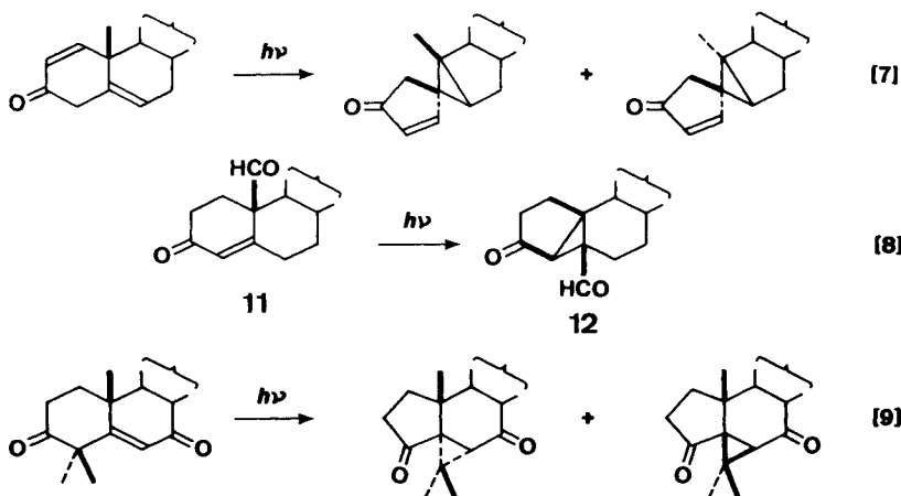
Scheme 2. Examples of Di- \pi -methane-type Rearrangements of Cyclohexenones Possessing Olefinic and Carbonyl \delta -Double Bonds
