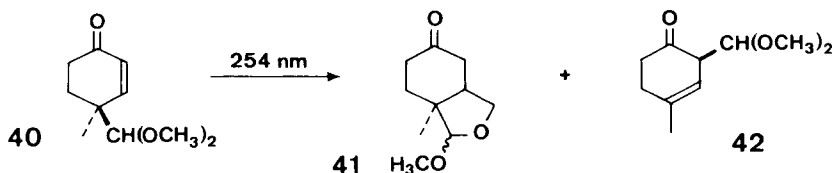
Scheme 8 14 )
