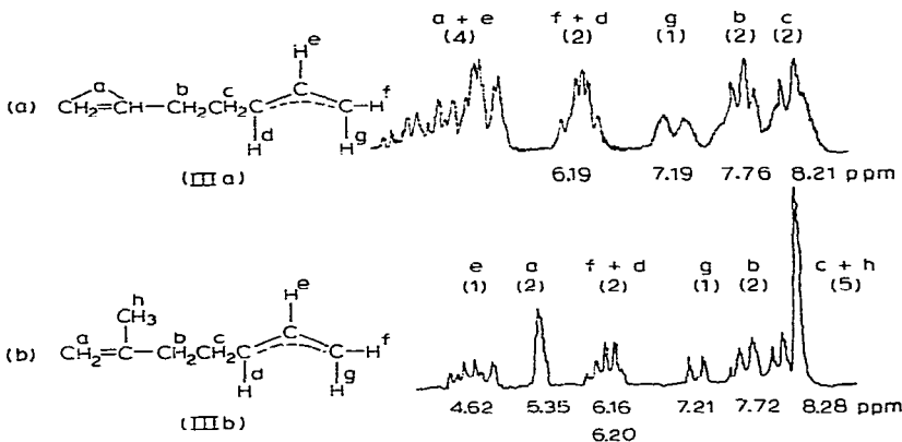
Fig. 1. NMR spectra of compounds (IIIa) and (IIIb) in carbon tetrachloride (internal standard TMS). The values in parentheses show intensity ratios. J_{eg} 12.0 Hz, J_{ef} 6.0 Hz.
