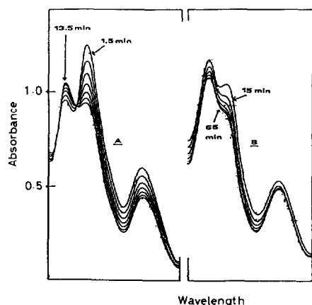
Fig. 3. UV-Vis spectrum of an aqueous solution of K_2-MoO_2S_2 ( 2.4 \times 10^{-4} M, pH 7.0, 30 °C) as a function of time. (a) 2 min scans over the period 1.5–15 min (note isobiestic point at 300 nm); (b) 10 min scans over the period 15–65 min. Both sets cover the range 260–440 nm (left to right).
