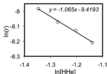
Figure 5. Initial formation rates of the InP nanoclusters vs the acid concentration (HHe). Reaction conditions: 0.4 mmol In(He) 3 , 0.2 mmol P(TMS) 3 , 4 mL ODE, T = 158 °C.
