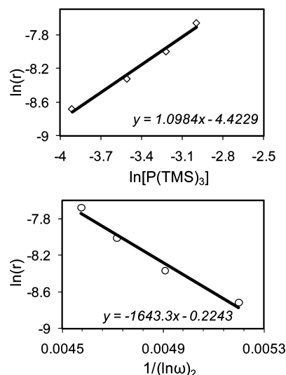
Figure 4. Initial formation rate of nanoclusters vs the concentration of limiting monomer, P(TMS)_3 . (Top) Plot as chemical kinetics. (Bottom) Plot as classic nucleation kinetics. Reaction conditions: 0.4 mmol In(He)_3 , 1.2 mmol HHe, 4 mL ODE, T = 158^\circ C .
