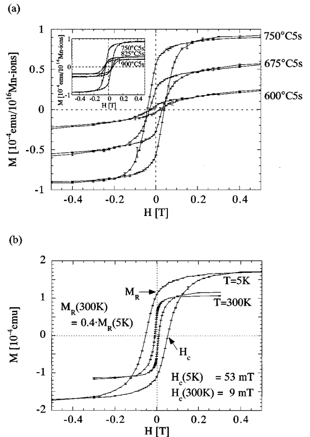
FIG. 2. (a) SQUID measurement at T=5 \text{ K} of the magnetization M(H) of LT-GaAs:Mn ( [Mn]=1 \cdot 10^{16} \text{ cm}^{-2} ) for various annealing conditions ( T=600-900 \text{ °C} , 5 s). The magnetization M(H) of each sample has been normalized to 10^{16} Mn ions. (b) SQUID measurement at 5 and 300 K of the magnetization M(H) of LT-GaAs:Mn annealed at 750 °C (180 s) ( [Mn]=1 \cdot 10^{16} \text{ cm}^{-2} ).
