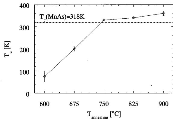
FIG. 3. Plot of the Curie temperature T_c of LT-GaAs:Mn ( [Mn]=1 \cdot 10^{16} \text{ cm}^{-2} ) vs the annealing temperature ( T=600\text{--}900^\circ\text{C} , 5 s).
