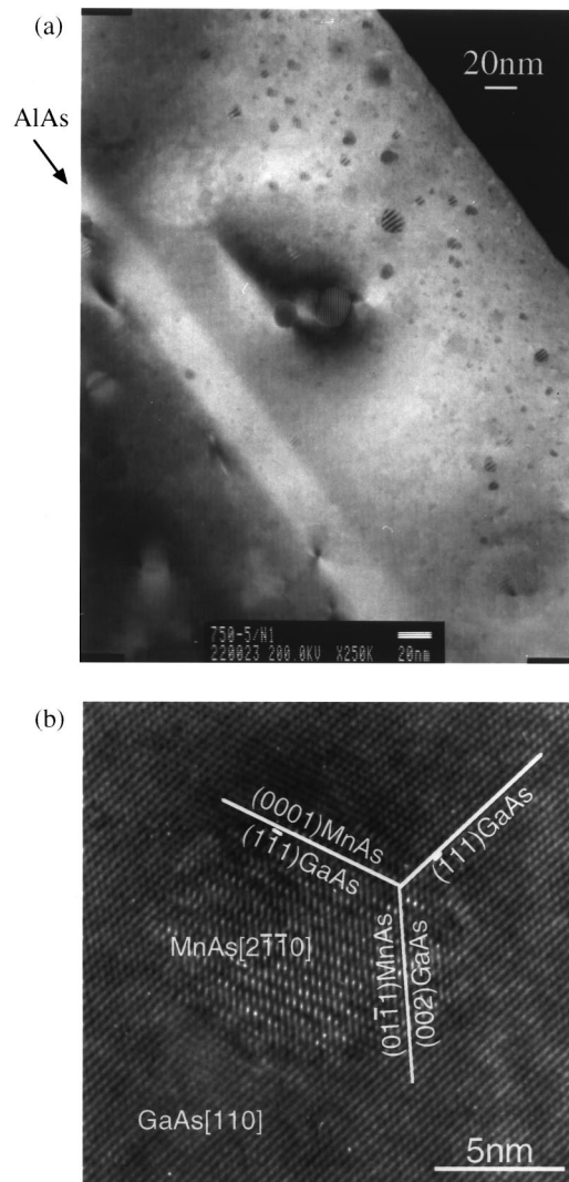
FIG. 1. (a) Cross sectional TEM image of LT-GaAs:Mn annealed at 750 °C (5 s) ( [\text{Mn}] = 1 \cdot 10^{16} \text{ cm}^{-2} ). (b) High resolution TEM image of a single MnAs crystallite in LT-GaAs:Mn annealed at 750 °C (5 s) ( [\text{Mn}] = 1 \cdot 10^{16} \text{ cm}^{-2} ).
