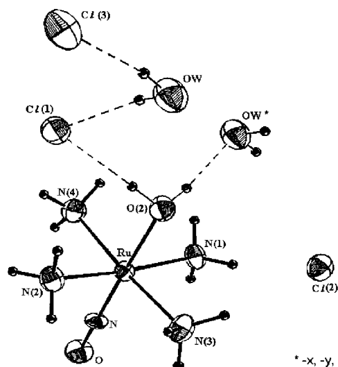
Figure 1. ORTEP representation with 50% of probability for [\text{Ru}(\text{NH}_3)_4(\text{H}_2\text{O})\text{NO}]\text{Cl}_3 \cdot \text{H}_2\text{O} .
