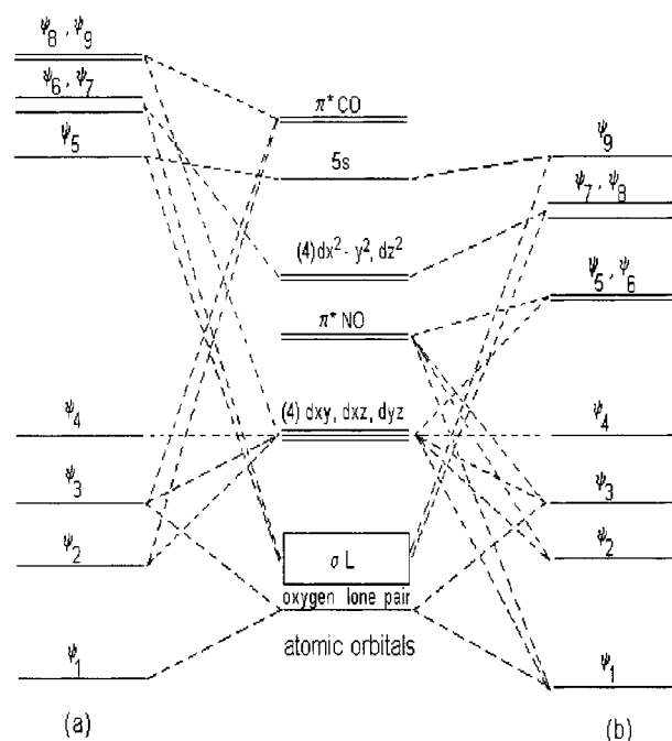
Figure 2. Relevant molecular orbitals and qualitative energy level scheme for (a) trans -[Ru(NH 3 ) 4 CO(H 2 O)]Cl 2 and (b) trans -[Ru(NH 3 ) 4 -NO(H 2 O)]Cl 3 .
