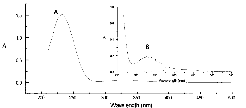
Figure 4. Electronic spectra of trans -[Ru(NH 3 ) 4 NO(H 2 O)]Cl 3 in 0.1 mol L -1 CF 3 COOH: (A) 6.5 \times 10^{-4} mol L -1 and (B) 9.6 \times 10^{-4} mol L -1 .
