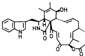
19- O -Acetylchaetoglobosin B ( 4 )
