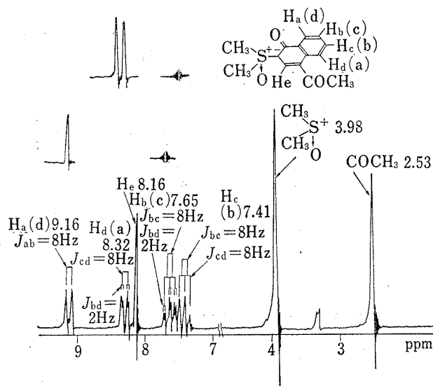
Fig. 1. NMR Spectrum of XII in \text{DMSO}-d_6 .
