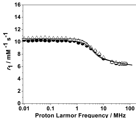
Fig. 3 ^1\text{H} NMRD profiles of Gd-5 (solid circles) and Gd-7 (open triangles). Data were recorded at 298 K and pH 6.8 and 6.7, respectively. The solid lines represent the best fitting results of the experimental data points with the parameters in Table 1.
