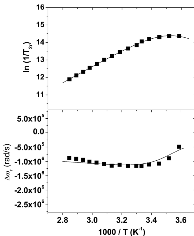
Fig. 4 Reduced transverse ^{17}\text{O} relaxation rates (above) and chemical shifts (below) measured at 11.74 T (pH 6.6) for Gd-7. The solid lines correspond to the fits of the data as described in the text.
