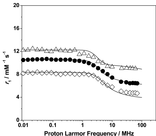
Fig. 5 ^1\text{H} NMRD profiles of Gd-7 at 283 K (open triangles), 298 K (solid circles) and 310 K (open diamonds) (pH 6.66).
