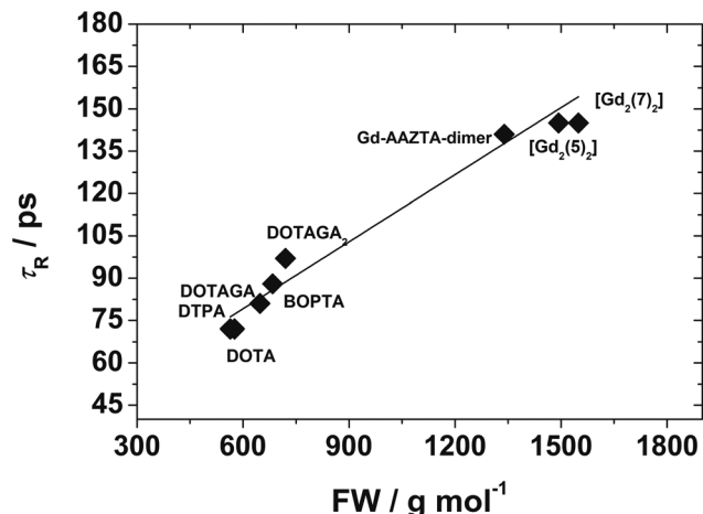
Fig. 6 Plot of the rotational correlation times of selected polyamino-carboxylate Gd-complexes as a function of molecular weight. The correlation coefficient R of the best fit line is 0.99. Data taken from ref. 24, 38 and 39 and this work.
