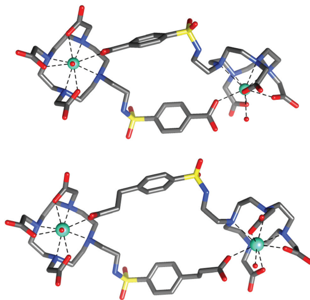
Fig. 7 Geometries of the TSAP conformers of [\text{Gd}_2(5)_2(\text{H}_2\text{O})_2] (top) and [\text{Gd}_2(7)_2(\text{H}_2\text{O})_2] (bottom), obtained from DFT calculations at the TPSSH/LCRECP/6-31G(d) level. For the corresponding SAP conformers see the ESI, Fig. S1†.
