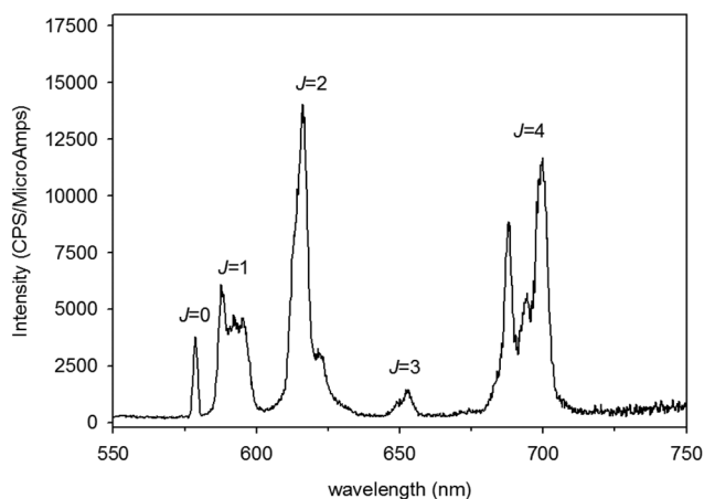
Fig. 2 Emission spectrum of the Eu-7 complex, recorded for a 1 mM solution under excitation at 395 nm ( \text{pH} = 7.2 ).
