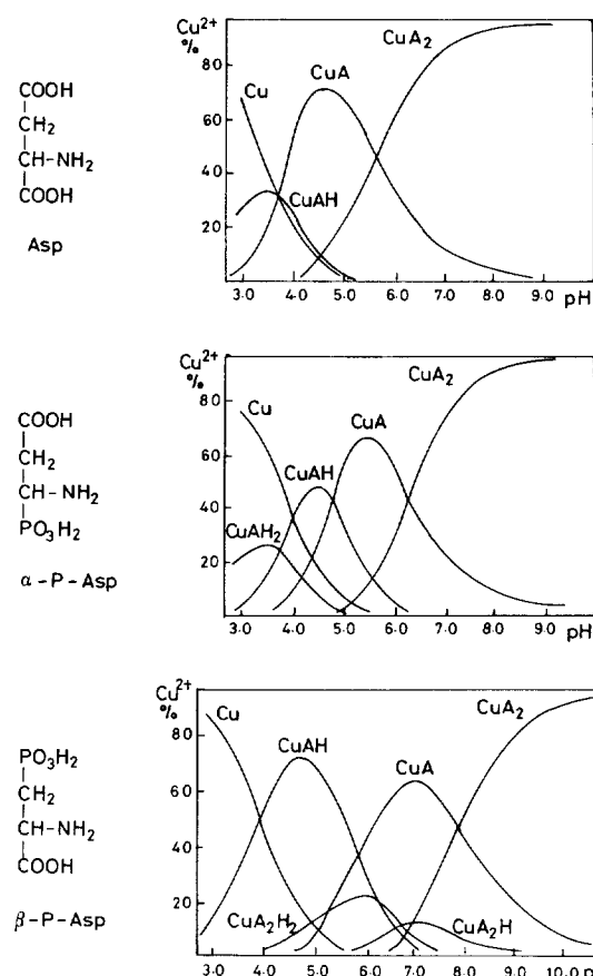
Fig. 2. Concentration distribution of the complexes formed in the copper(II)–Asp, copper(II)– \alpha -P-Asp and copper(II)– \beta -P-Asp systems as a function of pH. Details as in Fig. 1.
