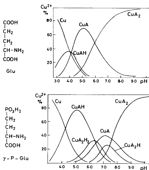
Fig. 1. Concentration distribution of the complexes formed in the copper(II)–Glu and copper(II)– \gamma -P-Glu systems as a function of pH. c_{\text{Cu}} = 0.002 , c_{\text{ligand}} = 0.004 mol dm -3 .
